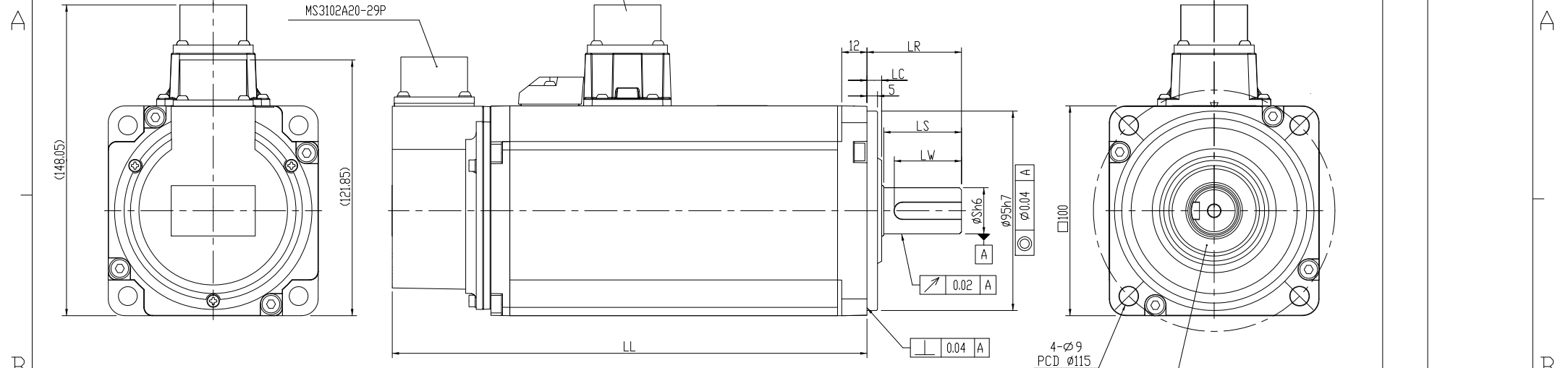
DIMENSION TABLE (MODEL WITH BRAKE)
