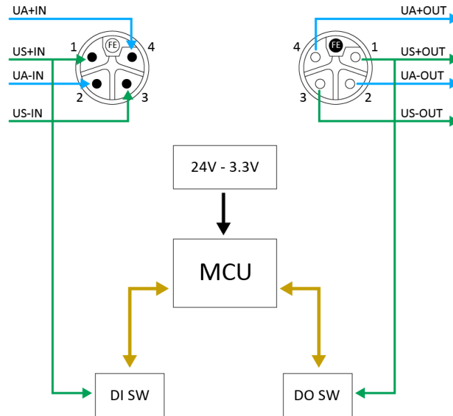
Typical connection diagram
